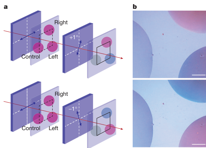
Figure 4 | Optical rotatory dispersion of self-assembled gold nanohelices. a , The macroscopic optical activity of the metafluid is demonstrated in polarization-resolved transmission by placing droplets of left-handed and right-handed nanohelices as well as a control droplet with isotropically dispersed gold nanoparticles between two linear polarizers. The components of the transmission set-up are ordered along the propagation path of white light as follows: linear polarizer, sample, linear analyser, screen (charge-coupled-device camera). The extinction characteristics of the linear polarizers render the set-up polarization-insensitive for wavelengths below 550 nm. b , Real-colour transmission images (scale bar, 1 mm) of the droplets for clockwise (top) and counter-clockwise (bottom) rotation of the analyser by one degree out of the orthogonal configuration. The droplets of right-handed and left-handed helices appear red in the top and bottom images, respectively, as a result of optical rotatory dispersion. Right- (or left-) handed nanohelices rotate the polarization axis of the transmitted light in positive (or negative) and negative (or positive) directions in the red and blue spectral bands, respectively. The rotation of the polarization in the red band is sensitively detected by the set-up, but green and blue components of white light illumination (below 550 nm) are not polarization-resolved and contribute only to the bluish background.
